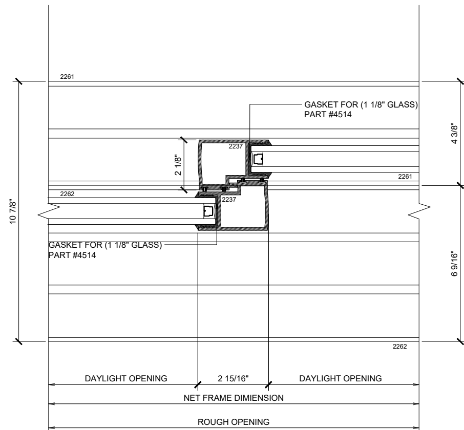
4 VERTICAL MAX SLIDING DOORS (OXXXX-XXXXO) SCALE: 6"=1'-0"
