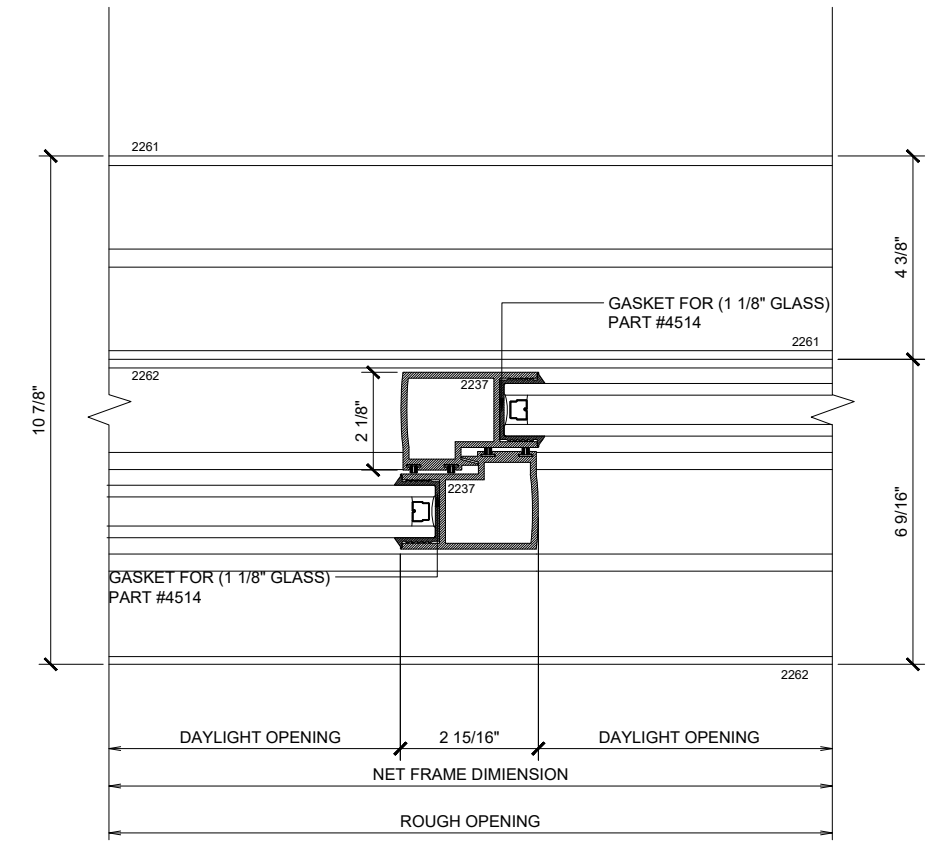
3 VERTICAL MAX SLIDING DOORS (OXXXX-XXXXO) SCALE: 6"=1'-0"
