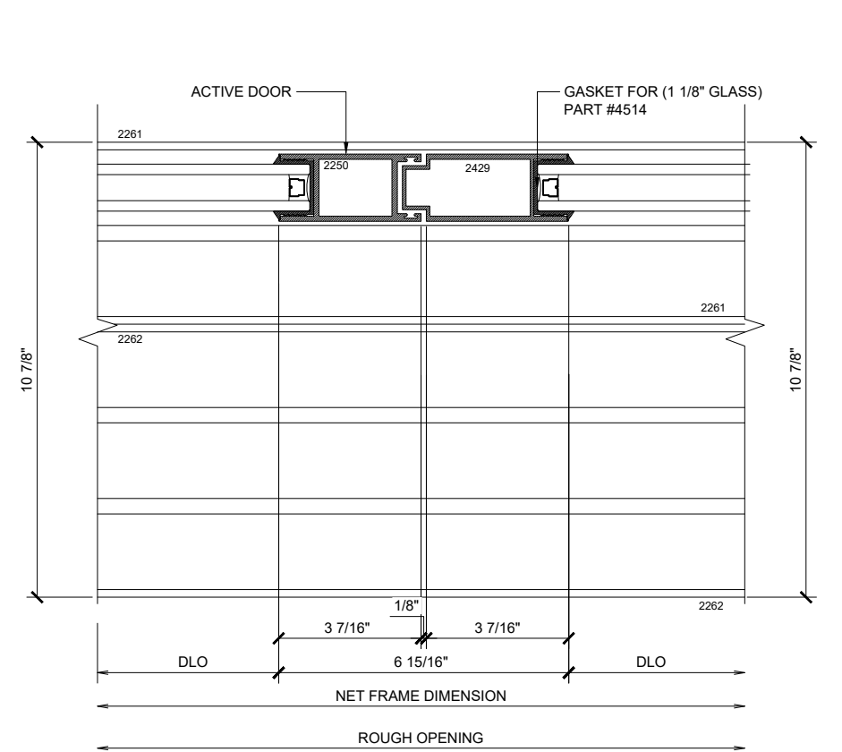
6 VERTICAL MAX SLIDING DOORS (OXXXX-XXXXO) SCALE: 6"=1'-0"
