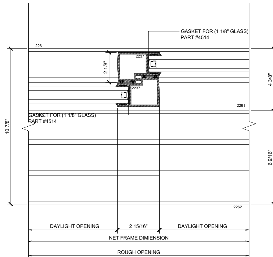
5 VERTICAL MAX SLIDING DOORS (OXXXX-XXXXO) SCALE: 6"=1'-0"
